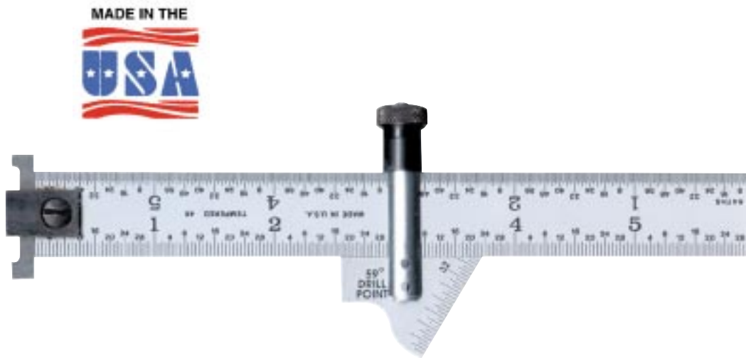
▲ Drill Point Gage #52-480-000
