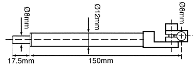
6" Swivel holder, 8mm
