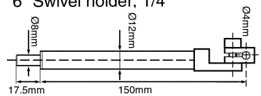
6" Swivel holder, 4mm
