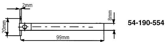
Measuring insert with interchangeable pin.
