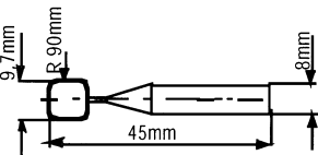
Barrel-shaped insert (M12-M150)
