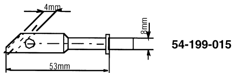
30° holder, Ø4mm
