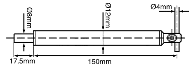
6" Probe holder, 4mm
