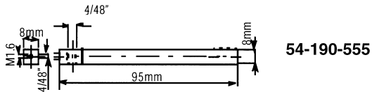
Measuring insert and insert for dial indicator probe
