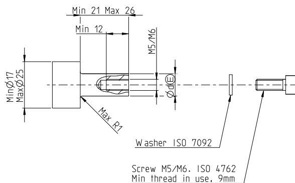
Dimensions [mm]
